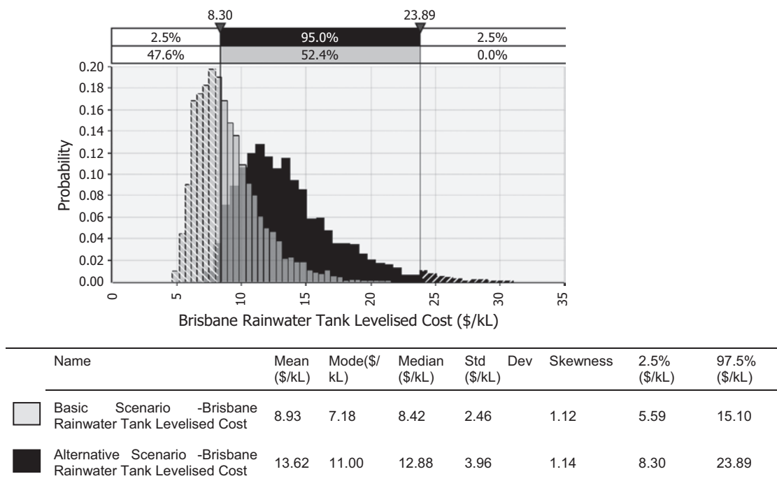
Figure 12.4 Brisbane rainwater tank cost-effectiveness probability density comparison of 'basic' and 'alternative scenario'.
