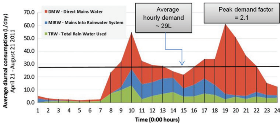
Figure 4.15 Diurnal water use pattern averaged over 4 months for one of the 20 households in the South East Queensland monitoring study.
