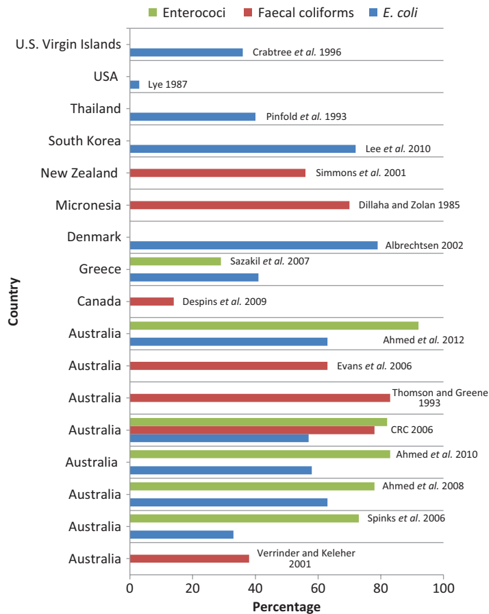
Figure 10.1 Percentage of samples positive for faecal indicators in tank water samples (Ahmed et al. 2011).
