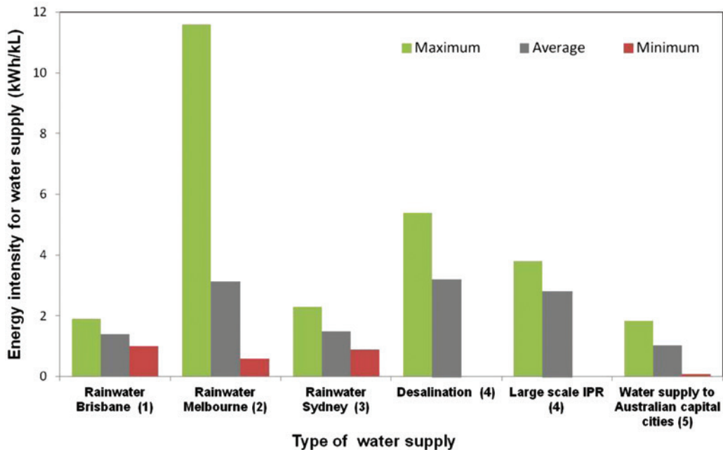
Figure 6.1 Examples of energy requirements for water delivery in major Australian capital cities. (Sources: (1) Gardner et al. (2006); (2) Hauber Davidson et al. (2010); (3) Retamal et al. (2009); (4) NSW Government (2006); (5) Kenway et al. (2008)).
