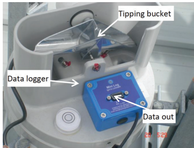
Figure 4.7 The internal tipping bucket and data logger of a typical pluviometer (for demonstration purposes only).
