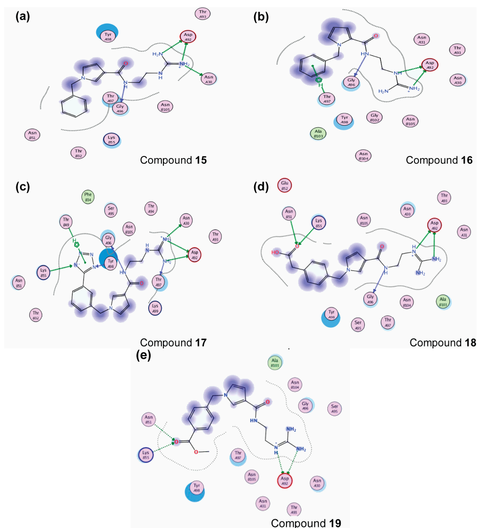
Figure 3. Best docking poses inside the TCR binding site, showing the different interactions for compounds: (a) 15; (b) 16; (c) 17, (d) 18; (e) 19. Green arrow: Hydrogen Bond (HB) formed with the side chain of the residue; Blue arrow: HB formed with the backbone; Blue shade: Solvent accessible surface area (SASA) of the ligand; Turquoise halo: SASA of the receptor residues; Green dotted lines: interaction of C-H with a \pi system (phenyl ring).
