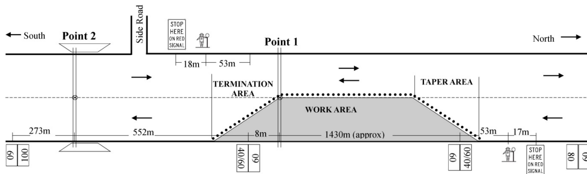
Figure 1. Plan of work zone
