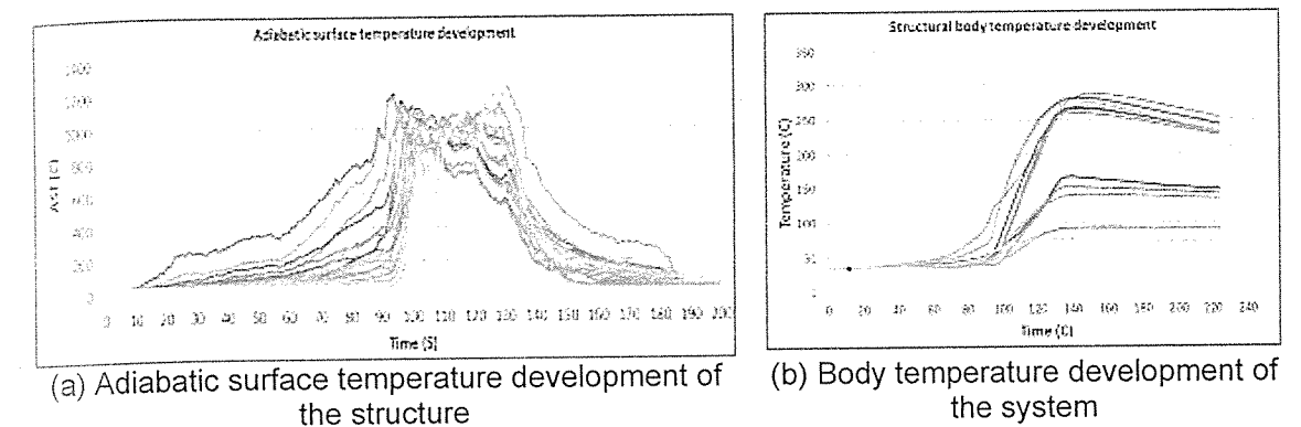
Figure 18. Surface and body temperature: Case A
