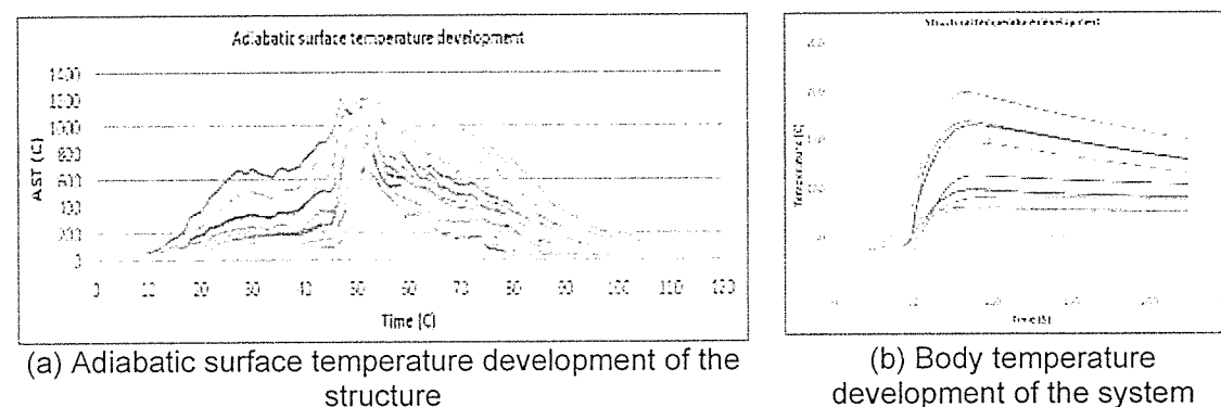
Figure 20. Surface and body temperature: Case B
