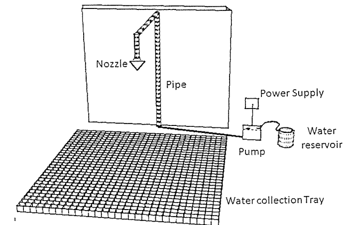
Figure 8: Schematic view of the experimental set-up from (Mahmud et al, 2016).
