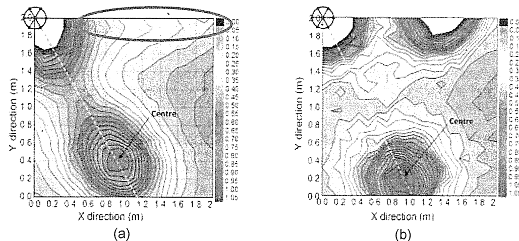
Figure 11: Distribution of flux density generated by a multi-orifice nozzle for case B; (a) Experimental, (b) Numerical.
