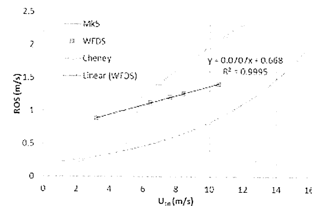
Figure 14: Effect of wind velocity on rate of spread (ROS)
