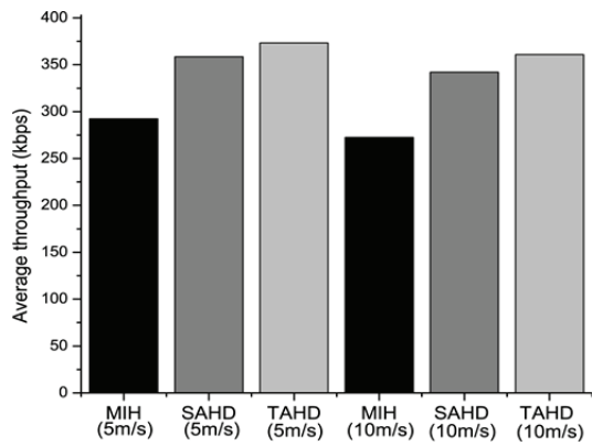
Fig. 13. Average throughput observed: Case 1.
