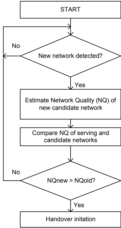
Fig. 8. Handover decision procedure in TAHD.
