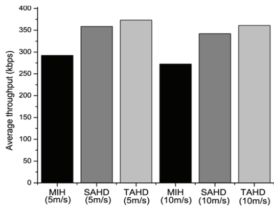
Fig. 14. Average throughput observed: Case 2.
