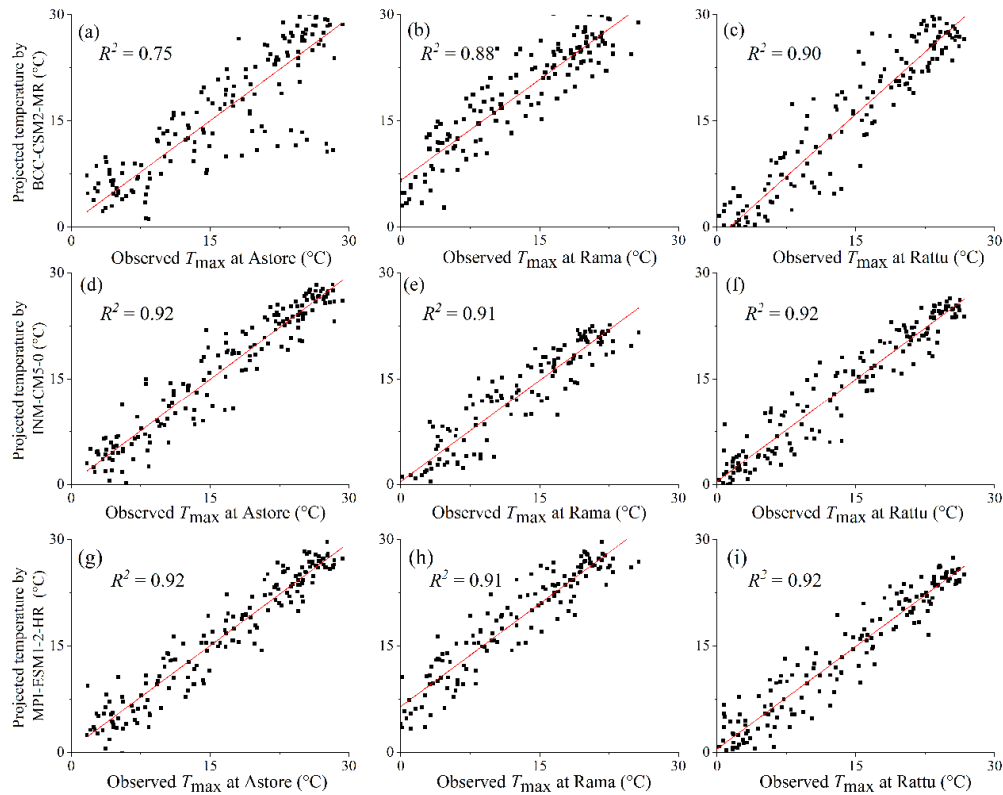
Fig. 6 Coefficient of Determination ( R^2 ) between observed daily maximum temperature and GCM (a-c) BCC-CSM2-MR, (d-f) INM-CM5-0 and (g-i) MPI-ESM1-2-HR during the period of 1995–2011.
