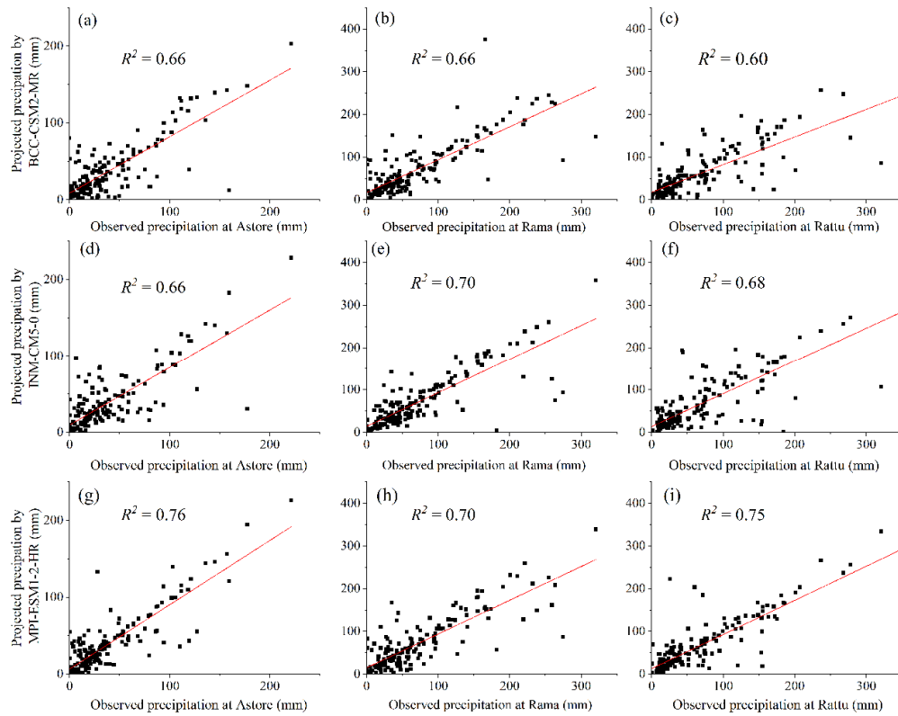
Fig. 5 Coefficient of determination ( R^2 ) between observed daily precipitation and GCM (a-c) BCC-CSM2-MR, (d-f) INM-CM5-0 and (g-i) MPI-ESM1-2-HR during the period of 1995–2011.
