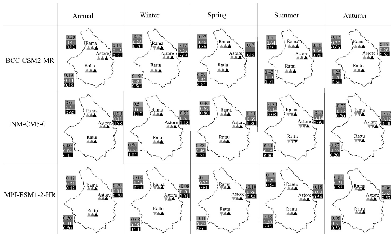
Fig. 9 Change in maximum temperature ( ^{\circ}\text{C}/\text{decade} ) under SSP1-2.6 (grey), SSP2-4.5 (dark grey) and SSP5-8.5 (black) scenarios at Astore, Rama and Rattu meteorological stations.
