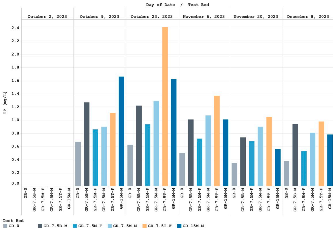
Figure 6. Total phosphorus (TP) concentration of runoff from different biochar–green roof test beds.
